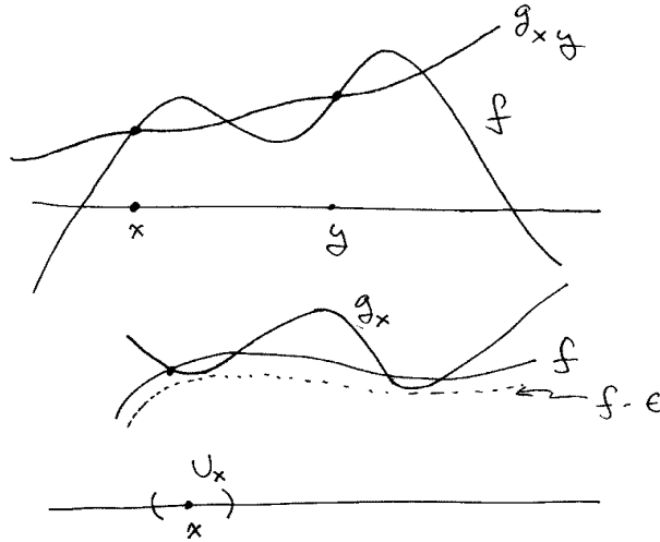
Fig. 12.6. Constructing the functions g_x .
