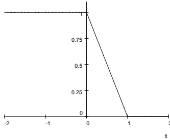
Fig. 12.3. The graph of the function \phi .
