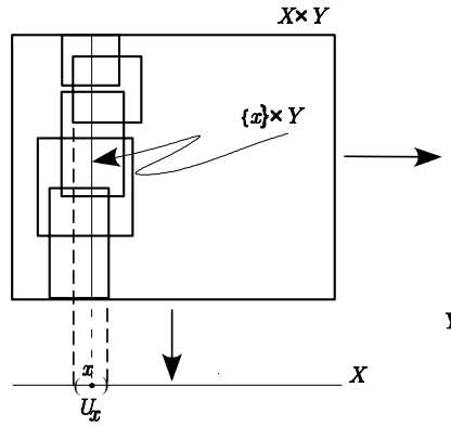
Fig. 11.4. Constructing the open set U_x .
