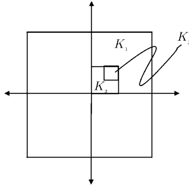
Fig. 11.3. Nested Sequence of cubes.
