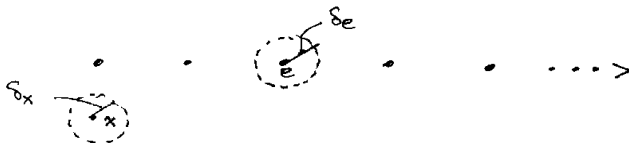
Fig. 11.1. The construction of an open cover with no finite sub-cover.
