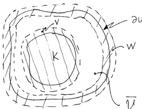
Fig. 12.1. The construction of V .
