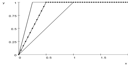
Fig. 22.1. The plot of \phi_n for n = 1, 2, and 4 . Notice that \phi_n \rightarrow 1_{(0,\infty)} .
