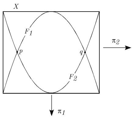
Fig. 14.5. Here \mathcal{F} = \{F_1, F_2\} where F_1 and F_2 are the two parabolic arcs and F_1 \cap F_2 = \{p, q\} .
