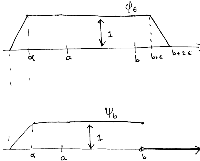
Fig. 29.3. A couple of functions in \overline{S_c(\mathcal{A})} .
