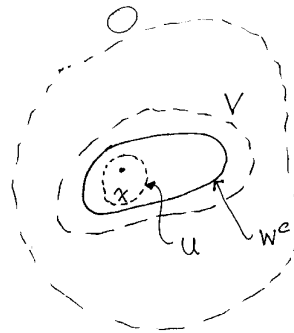
Fig. 15.7. Constructing (U, V) \in \Gamma .
