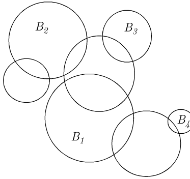
Fig. 29.1. Picking out the large disjoint balls.
