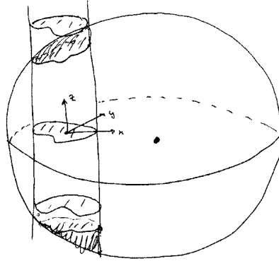
Fig. 35.3. The geometry of the solution to the wave equation in two dimensions.
