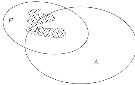
Fig. 19.1. Completing a \sigma -algebra.
