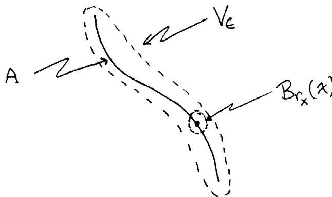
Fig. 29.2. Covering a small set with balls.
