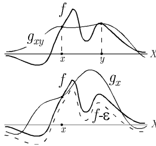
Fig. 15.6. Constructing the “dominating approximates,” g_x for each x \in X .
