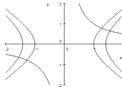
Fig. 20.3. The region \Omega consists of the two curved rectangular regions shown.
