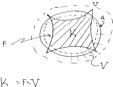
Fig. 28.1. Constructing the compact set K .
