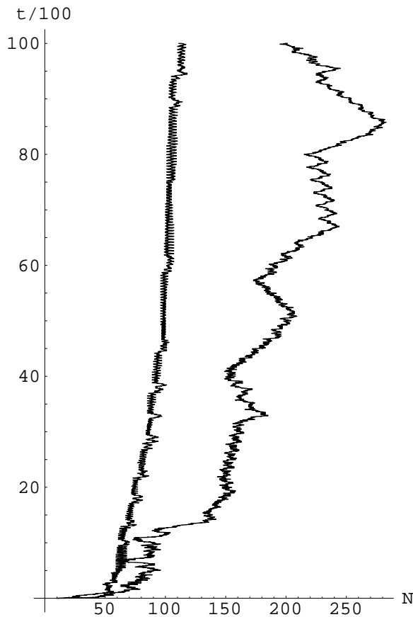
Figure 8. Lattice sizes for simulations of 10000 timesteps from initial configurations of 10 and 17 particles on a lattice of size 10. Time runs upward and the graph of (mostly) smaller sizes is the 10 particle simulation.
