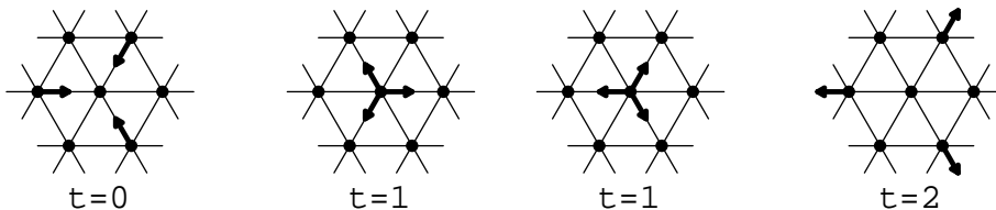
Figure 4. The zero momentum three particle scattering rule in the FHP model. Advection takes the t = 0 configuration to the the first t = 1 configuration shown; then the scattering rule changes that to the second t = 1 configuration; advecting again (followed by scattering, which has no effect) produces the t = 2 configuration.
