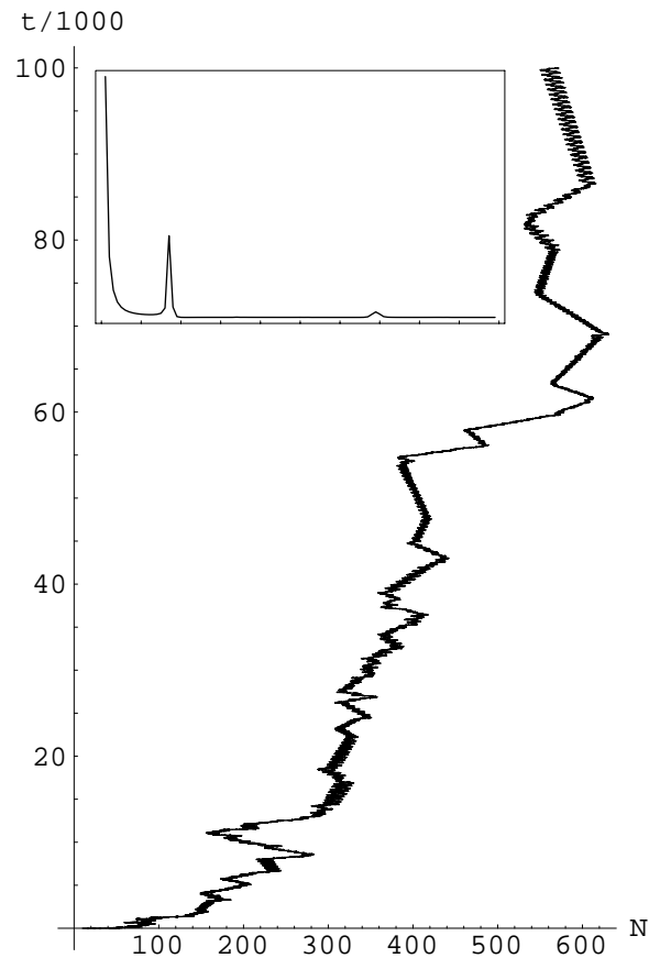
Figure 9. The 17 particle simulation extended to 100000 timesteps. The insert shows the norm squared of the first 100 Fourier coefficients (the ticks are at multiples of 20) calculated for the last 10000 sizes in the time series.
