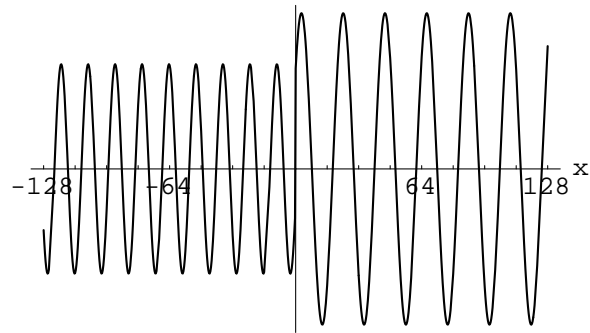
Figure 9. The eigenfunction of U in the same situation as in Figures 7 and 8, but now for an even taller step, of height 7\pi/24 . Rather than decaying even faster than in Figure 8, the amplitude of the wave function oscillates to the right of the step, with wave number approximately 0.296.
