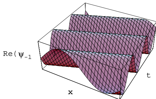
Figure 4. Evolution of the k = \pi/16 right moving plane wave for the interval 0 \leq x \leq 31 when \theta = \pi/12 .
