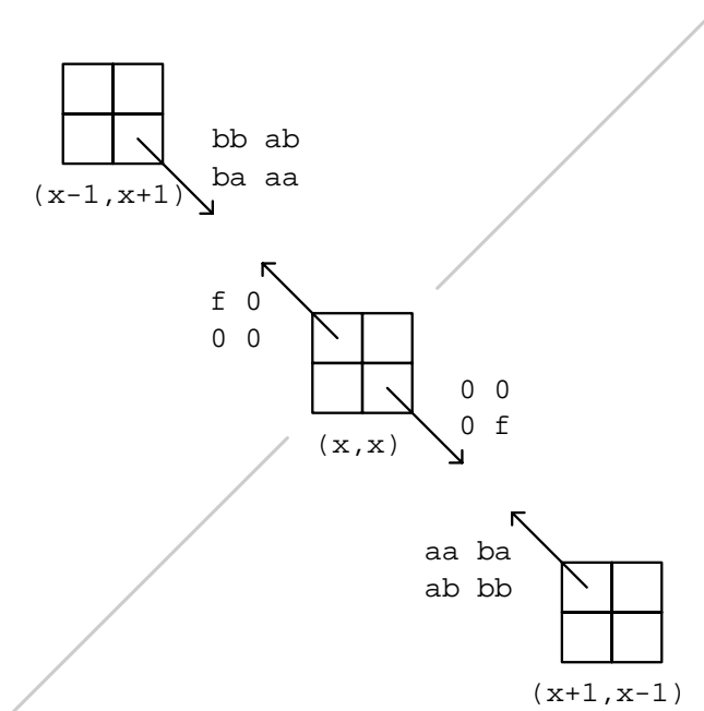
Figure 11. Schematic diagram of a subspace of H_{2,\text{int}} . The coordinates x_1 and x_2 of the two particles label the sets of four boxes, each of which corresponds to a pair of ‘velocities’. The evolution rule (4.4) gives the amplitude flows shown pointing toward the diagonal (where the particles coincide), while (4.5) gives the amplitude flows shown pointing away from it. In order for the ansatz (4.9) to satisfy (4.7) for x_1 \neq x_2 , the amplitude flows away from the diagonal must satisfy (4.10); in order for it to satisfy (4.11) the amplitude flows toward the diagonal must satisfy (4.12).
