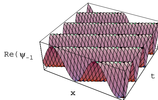
Figure 5. The same simulation for the k = \pi/8 right moving plane wave. This wave has a higher frequency.
