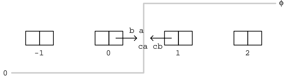
Figure 6. Schematic diagram of a subspace of H_1 when there is a potential step of height \phi between x = 0 and x = 1 . As in Figure 2, the boxes represent dimensions of the Hilbert space and the labelled arrows indicate the amplitude flow (here c := e^{-i\phi} ). Equations (3.8) correspond to the statements that the left moving amplitude flow from x = 1 equals what it would be were the ansatz for x \leq 0 continued to x = 1 , and that the right moving amplitude flow from x = 0 equals what it would be were the ansatz for x \geq 1 continued to x = 0 , respectively.
