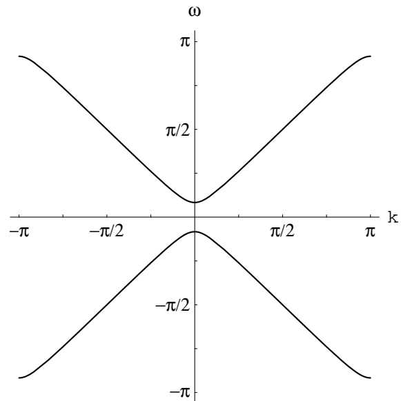
Figure 3. The dispersion relation for \theta = \pi/12 . There are two branches and a frequency gap between \theta and -\theta .
