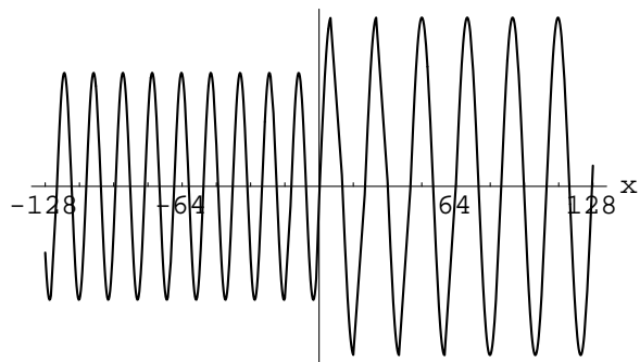
Figure 7. The real part of the \alpha = -1 component of an eigenfunction of U with frequency \omega = \pi/6 for a step of height \pi/24 with \theta = \pi/12 on the interval -128 \leq x \leq 128 . This wave function has wave numbers approximately 0.459 to the left of, and 0.296 to the right of the step.
