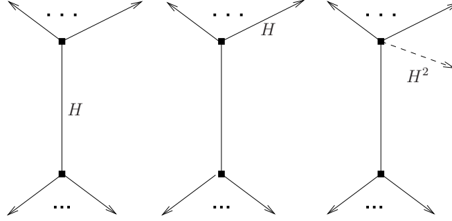
FIGURE 10. The codimension 2 tautological generators for graphs with two vertices.
