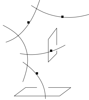
FIGURE 1. The tautological generators [\Gamma, \mathfrak{w}, \mathfrak{f}] .
