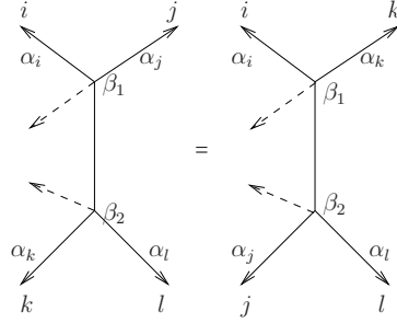
FIGURE 9. Generalized Keel relations.
