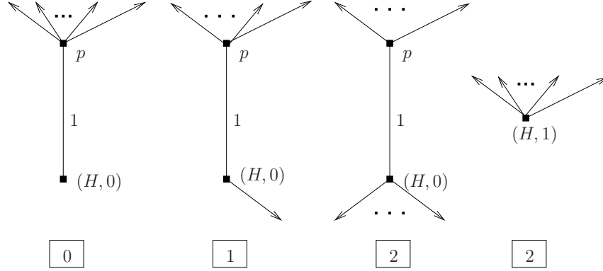
FIGURE 11. The fixed loci on \overline{\mathcal{M}}_{0,n}(\mathbb{P}^r, 1) .
