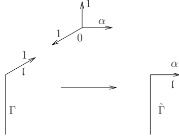
FIGURE 8. Adding in weights via gluing and forgetting.
