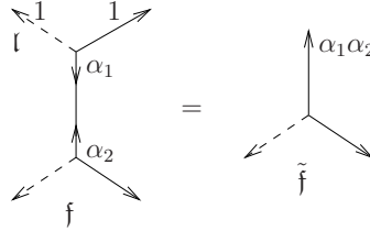
FIGURE 5. Forgetting destabilizing legs
