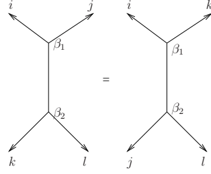
FIGURE 6. The pullbacks of Keel relations.
