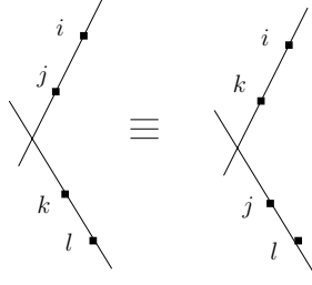
FIGURE 3. Keel's relations on \overline{\mathcal{M}}_{0,n} .
