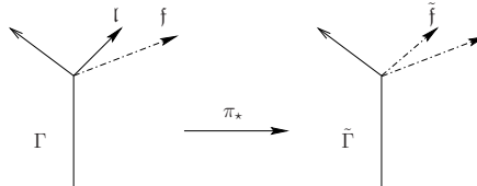
FIGURE 4. The forgetting maps
