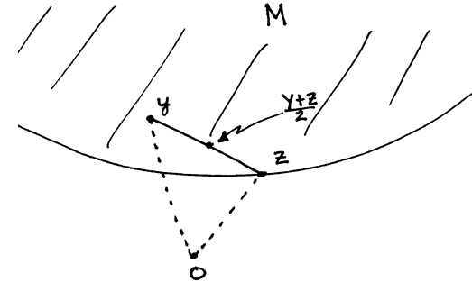
Fig. 16.2. The geometry of convex sets.
