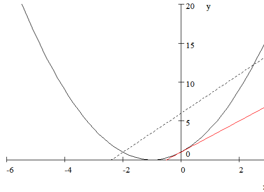
Fig. 7.2. A convex function, \varphi , along with a cord and a tangent line. Notice that the tangent line is always below \varphi and the cord lies above \varphi between the points of intersection of the cord with the graph of \varphi .
