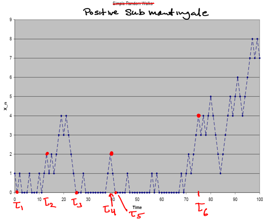
Fig. 19.2. A sample path of a positive submartingale along with stopping times \tau_{2j} and \tau_{2j+1} , successive hitting times of 2 and 0 respectively.
