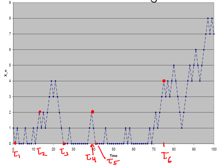
Fig. 19.2. A sample path of a positive submartingale along with stopping times \tau_{2j} and \tau_{2j+1} , successive hitting times of 2 and 0 respectively.
