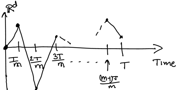
Fig. 23.2. A typical path in W_{m,T} .
