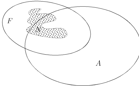
Fig. 5.1. Completing a \sigma -algebra.
