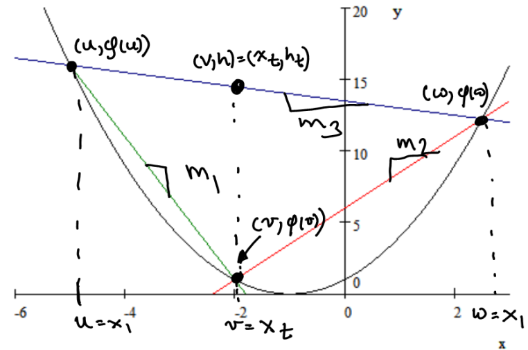
Fig. 11.1. A convex function with three chords. Notice the slope relationships; m_1 \leq m_3 \leq m_2 .
