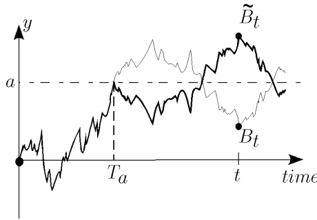
Fig. 24.3. The Brownian motion B_t and its reflection \tilde{B}_t about the line y = a . Note that after time T_a , the labelings of the B_t and the \tilde{B}_t could be interchanged and the picture would still be possible. This should help alleviate the readers fears that Brownian motion has some funny asymmetry after the first hitting of level a .
