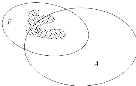
Fig. 5.1. Completing a \sigma -algebra.
