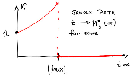
Fig. 25.2. A typical sample path of M_t^0(x) .
