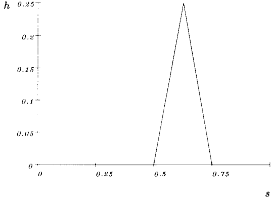
FIGURE 1. This function is a typical element of V_3 . It is the function h_3 as described in Lemma 6.24 with n = 3 .
