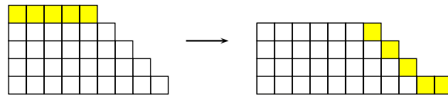
Figure 7.8: Case 2b: t(\lambda) \leq s_1(\lambda) \Leftrightarrow 1
